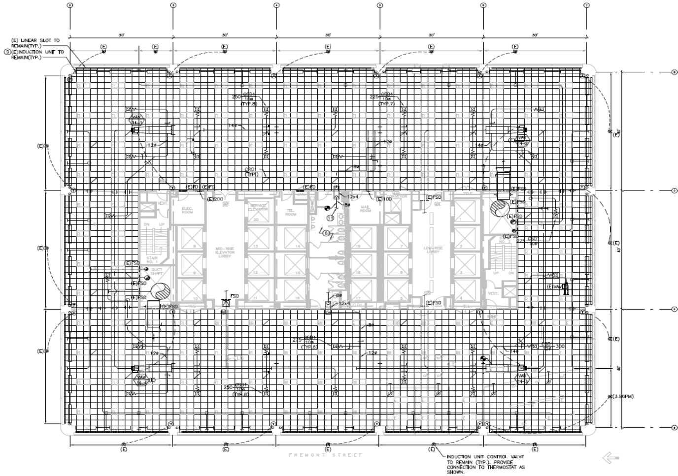
1 14TH FLOOR - MECHANICAL FLOOR PLAN SCALE: 1/8"=1'-0"
